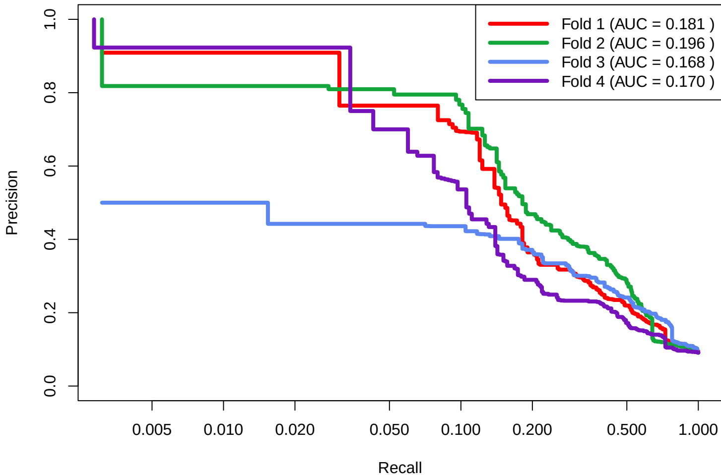
SPELL All Datasets: 430x50x20x10x1 Validation
